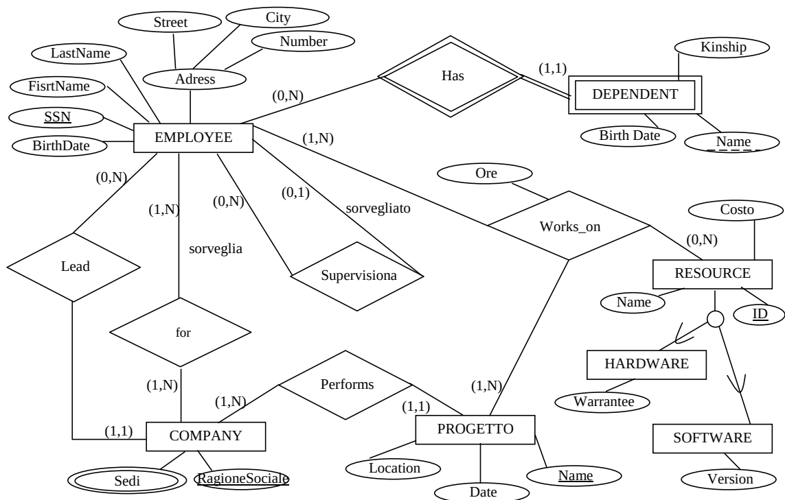
Figure 1: The ER diagram of a system managing company information
